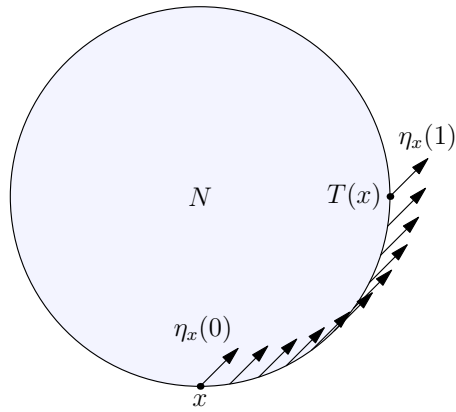
Figure 4.2: Values of \eta_x from 0 to 1
