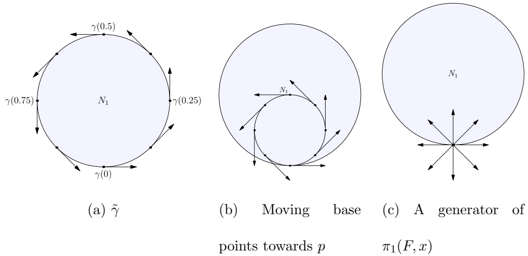
Figure 3.2: \tilde{\gamma} is homotopic to a generator of \pi_1(F, x)
