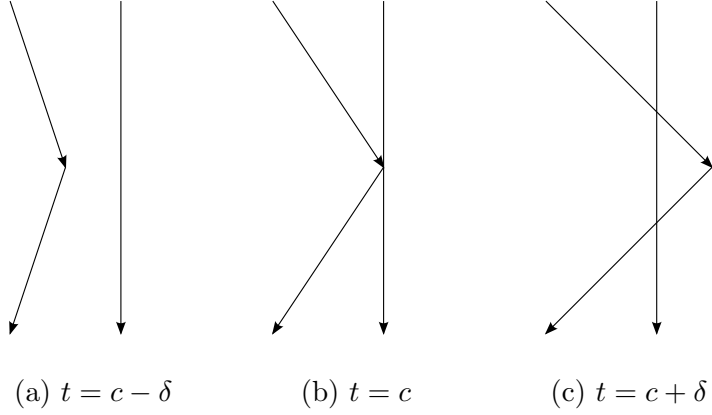
Figure 3.6: 3.6c has two more crossing of the same type but opposite signs compared to 3.6a. This corresponds to a Reidemeister move of type II.
