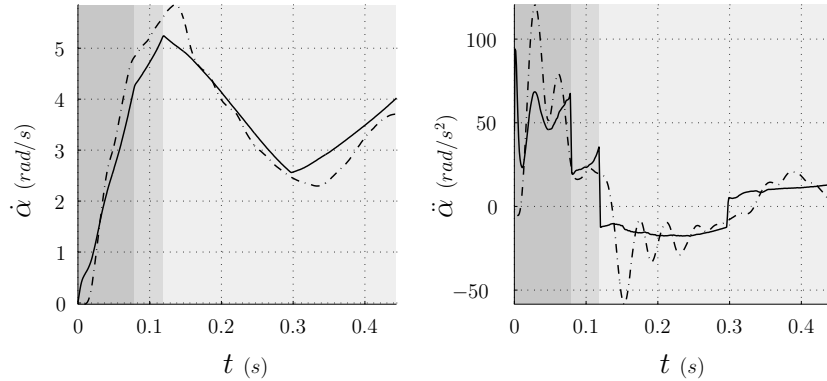
Fig. 7. Model predictions for the pitch velocity(left) and acceleration(right) compared to the experiment with best model performance ( \mu_t = 0.39 ). Solid lines indicate model prediction whereas dashed lines show the actual measurements. Shaded regions indicate different number of legs in contact with the ground: dark(3), middle(2) and light(1)
