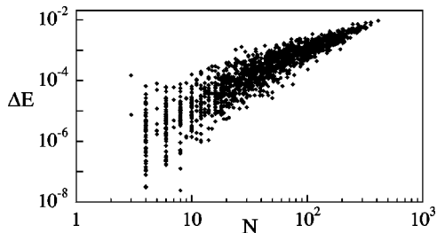
FIG. 4. The size of energy drops as a function of the number of bubbles that concurrently change overlapping neighbors during the energy drop, for a 900-bubble system at \phi=1.0 driven at \dot{\gamma}=10^{-3} . This indicates that the fraction of bubbles that change overlapping neighbors during an energy drop increases with the size of the energy drop.
