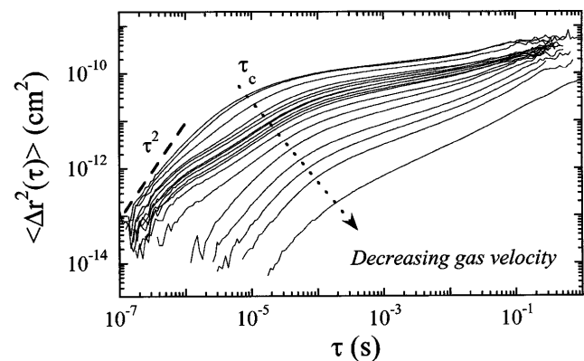
FIG. 2. DWS results for mean square displacement of beads, \langle \Delta r^2(\tau) \rangle (in \text{cm}^2 ), as a function of time, \tau (in \text{sec} ) in a bed of 96 \mu\text{m} beads. The short time dynamics are collisional with \langle \Delta r^2(\tau) \rangle = \delta V^2 \tau^2 for \tau < \tau_c , the collision time. As U_s is increased, the collisional regime shifts to shorter times and higher velocities. For \tau > \tau_c , \langle \Delta r^2(\tau) \rangle changes very slowly with \tau for several decades in time.
