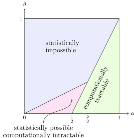
FIG. 1. Detection boundary \beta^* versus efficiently computable detection boundary \beta^\# .
