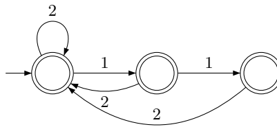
Fig. 2. A deterministic Büchi automaton for MaxCon(1, 2) .
