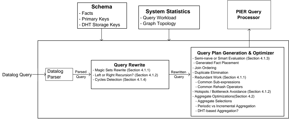
Figure 5: Datalog Query to Optimized Query Plan.
