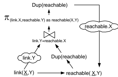
Figure 6: Query Execution Plan for the Reachable Program.
