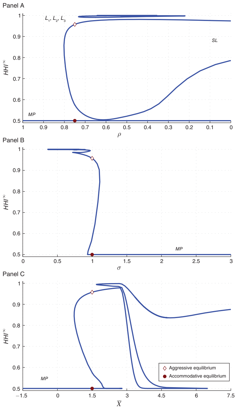
FIGURE 2. EQUILIBRIUM CORRESPONDENCE
