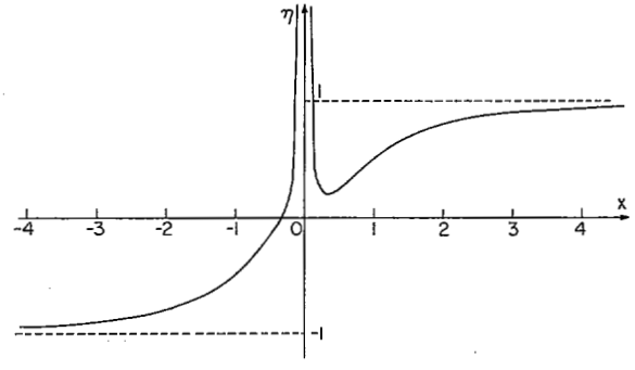
Fig. 5. Function \eta(X) for transverse magnetic field as measured by an observer moving at velocity v with respect to dipole oscillating at frequency \omega = kc in K , where X \equiv kv't' = kv't and \beta = 1/100 . In general, \eta(0) = 1/\beta .
