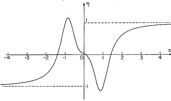
Fig. 4. Function \eta(X) for transverse electric field as measured by an observer moving at velocity v with respect to dipole oscillating at frequency \omega = kc in K , where X \equiv kv't' = kv't and \beta = 1/100 .
