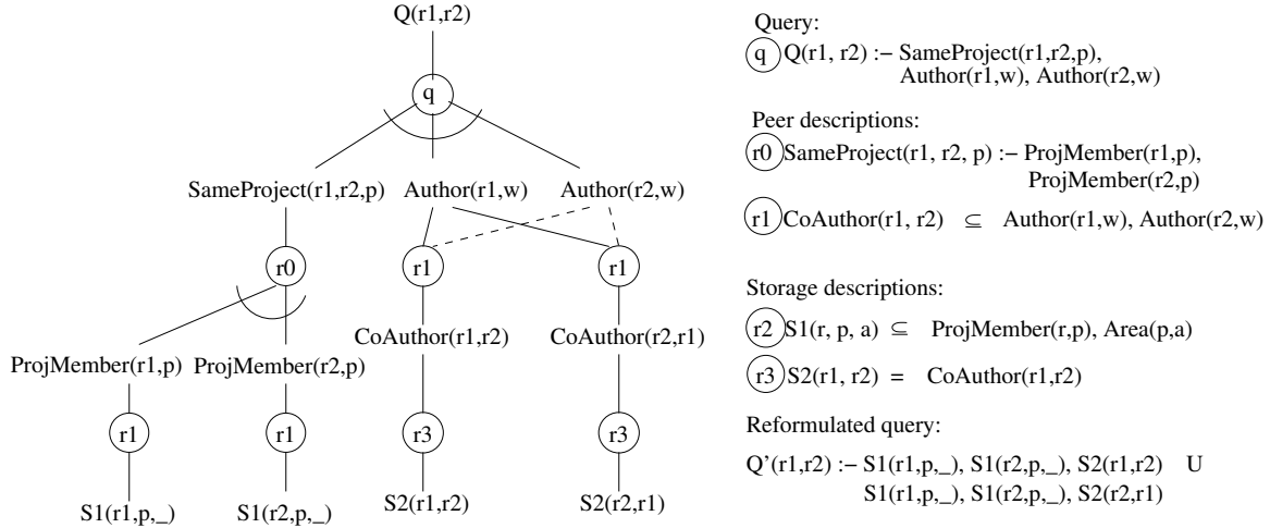
Fig. 2 Reformulation rule-goal tree for the database research domain. Dashed lines represent nodes that are included in the unc label (see text).
