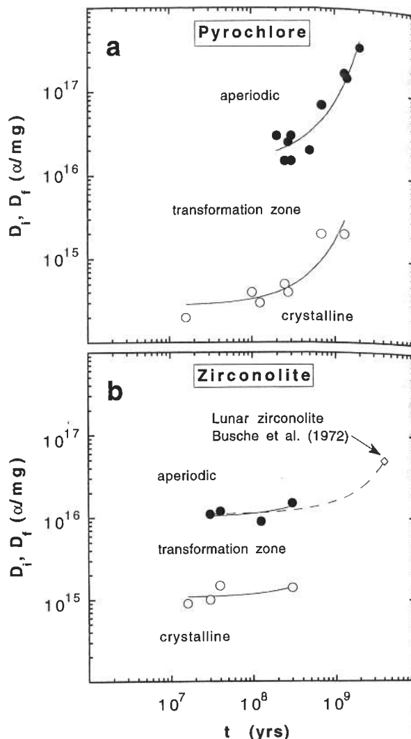
Fig. 1. Plots of alpha-decay dose in \alpha/\text{mg} versus geologic age showing data which define the beginning (initial dose, D_i ) and end (final dose, D_f ) of the crystalline-aperiodic transformation for a) pyrochlore and b) zirconolite.
