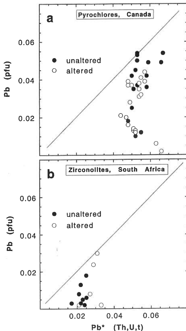
Fig. 3. EPMA data showing the measured Pb content plotted versus Pb*, the expected amount of radiogenic Pb from the decay of Th and U over time, for radiation damaged samples of a) pyrochlore from Canada (age = 1.0 \times 10^9 yr, dose = 5-8 \times 10^{17} a/mg) and b) zirconolite from South Africa (age = 2.5 \times 10^9 yr, dose = 2-3 \times 10^{17} a/mg).
