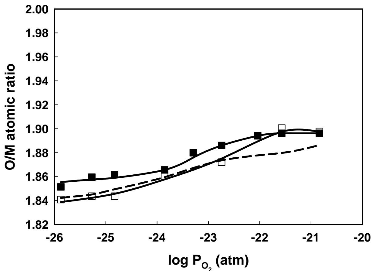
Figure 7c). O/M ratios as a function of P(\text{O}_2) for the \text{Ce}_{0.33}\text{Zr}_{0.67}\text{O}_2 sample after calcination for 4 hours at 973 K (□) and 1323 K (■). The simulated result (---) was calculated by assuming the sample calcined to 1323 K could be modeled as a physical mixture of \text{Ce}_{0.81}\text{Zr}_{0.19}\text{O}_2 and \text{Ce}_{0.25}\text{Zr}_{0.75}\text{O}_2 .
