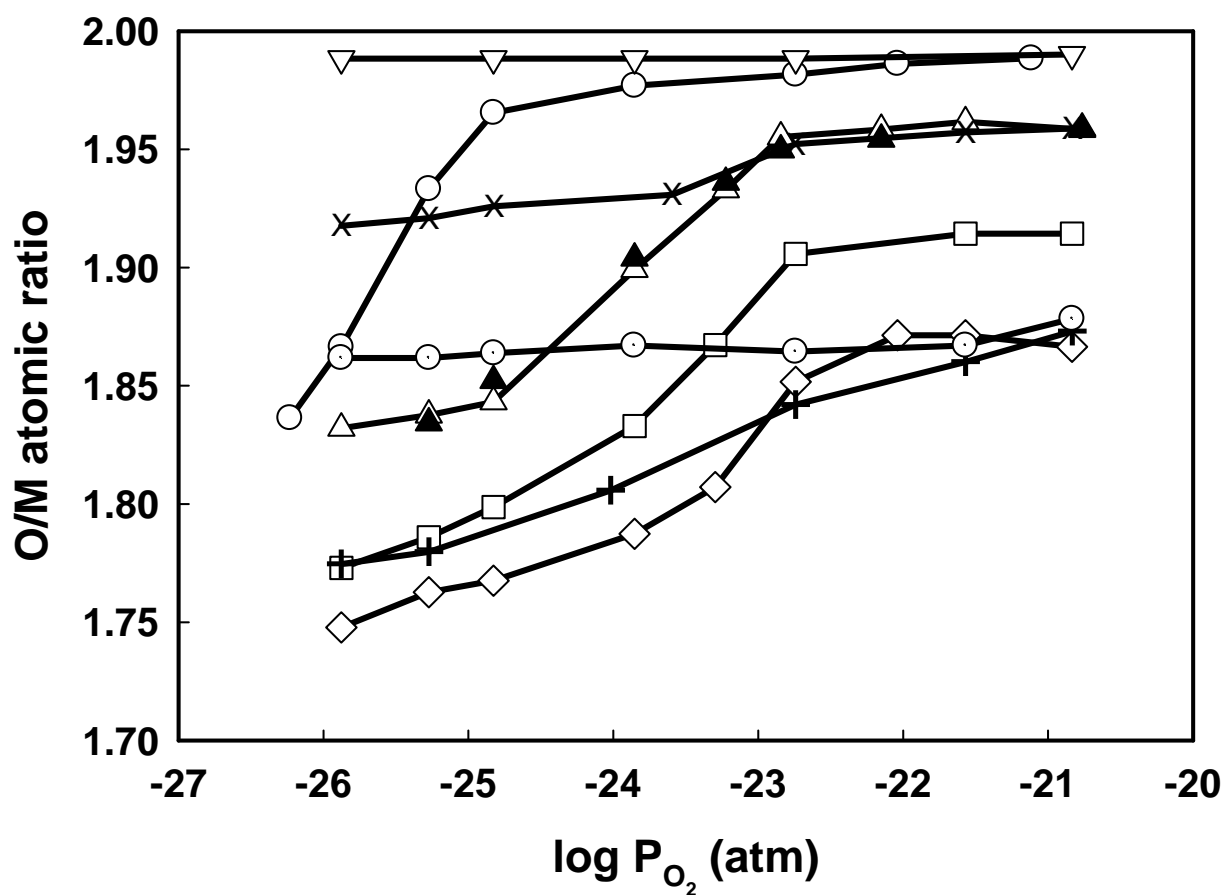
Figure 3. Oxygen to total metal (Ce+Zr) ratios for the Ce_yZr_{1-y}O_{2-x} samples, following calcination at 973 K, as a function of P(O_2) . The y values in the samples are as follows: (○) y=1 , ( \Delta ) y=0.92 , ( \square ) y=0.81 , ( \diamond ) y=0.59 , (+) y=0.5 , ( \ominus ) y=0.25 , (x) y=0.14 , and ( \nabla ) y=1.0 . The closed symbols for y=0.08 ( \blacktriangle ) were obtained from the sample after calcination at 1323 K for 4 h.
