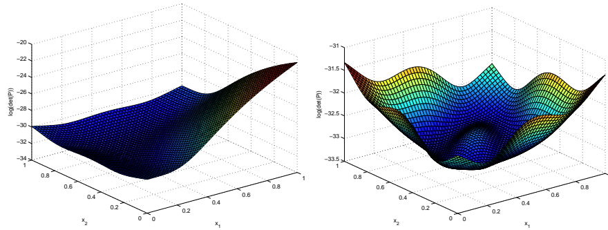
Fig. 8. (a) Uncertainty of position estimates under sensing graph \mathcal{G}_1 . (b) Uncertainty of position estimates under sensing graph \mathcal{G}_2 .
