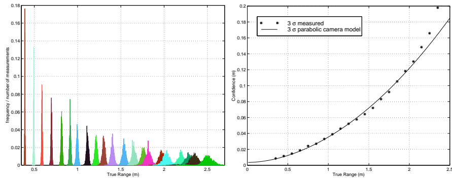
Fig. 5. (a) Omni-directional camera measurements and feature range histogram. (b) Measured and modeled range measurement uncertainty
