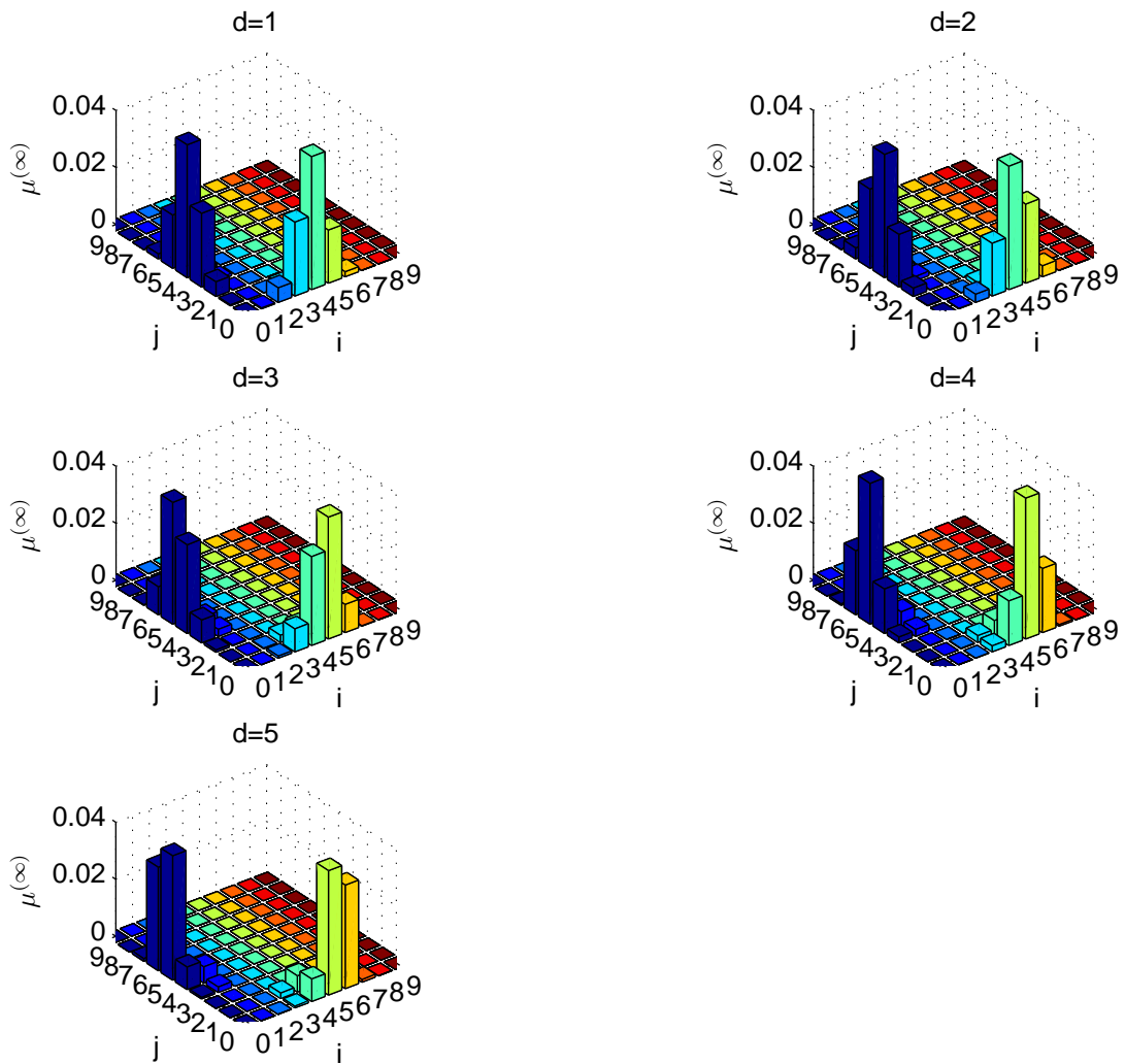
Figure 2: Limiting distribution \mu^{(\infty)} . First equilibrium.
