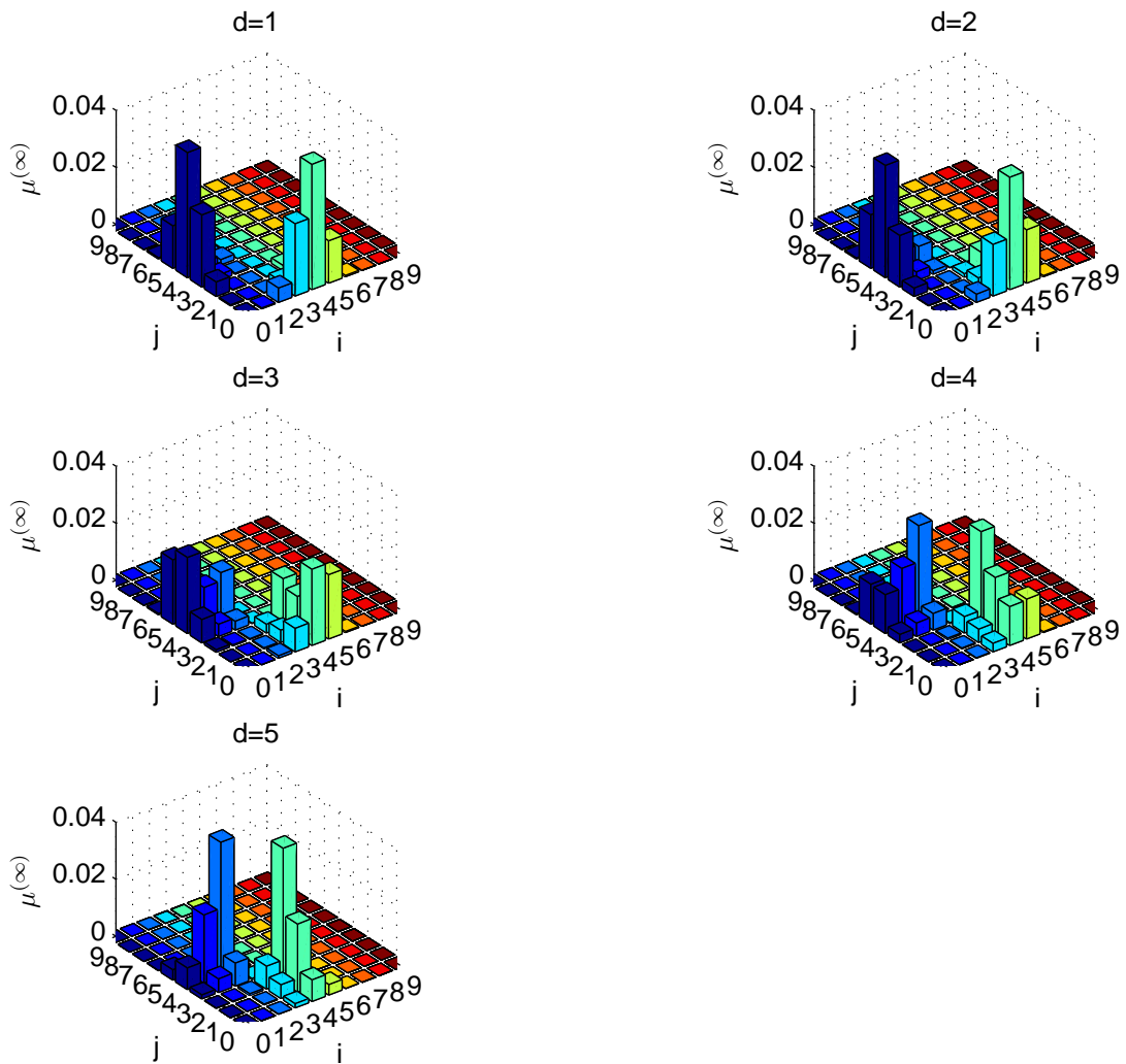
Figure 4: Limiting distribution \mu^{(\infty)} . Third equilibrium.
