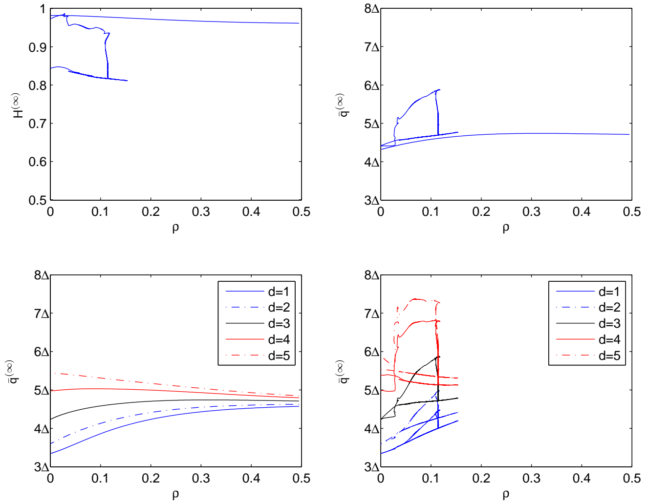
Figure 1: Herfindahl index of firms' capacities H^{(\infty)} (top left panel) and total capacity \bar{q}^{(\infty)} unconditional (top right panel) and conditional on state of demand (bottom panels).
