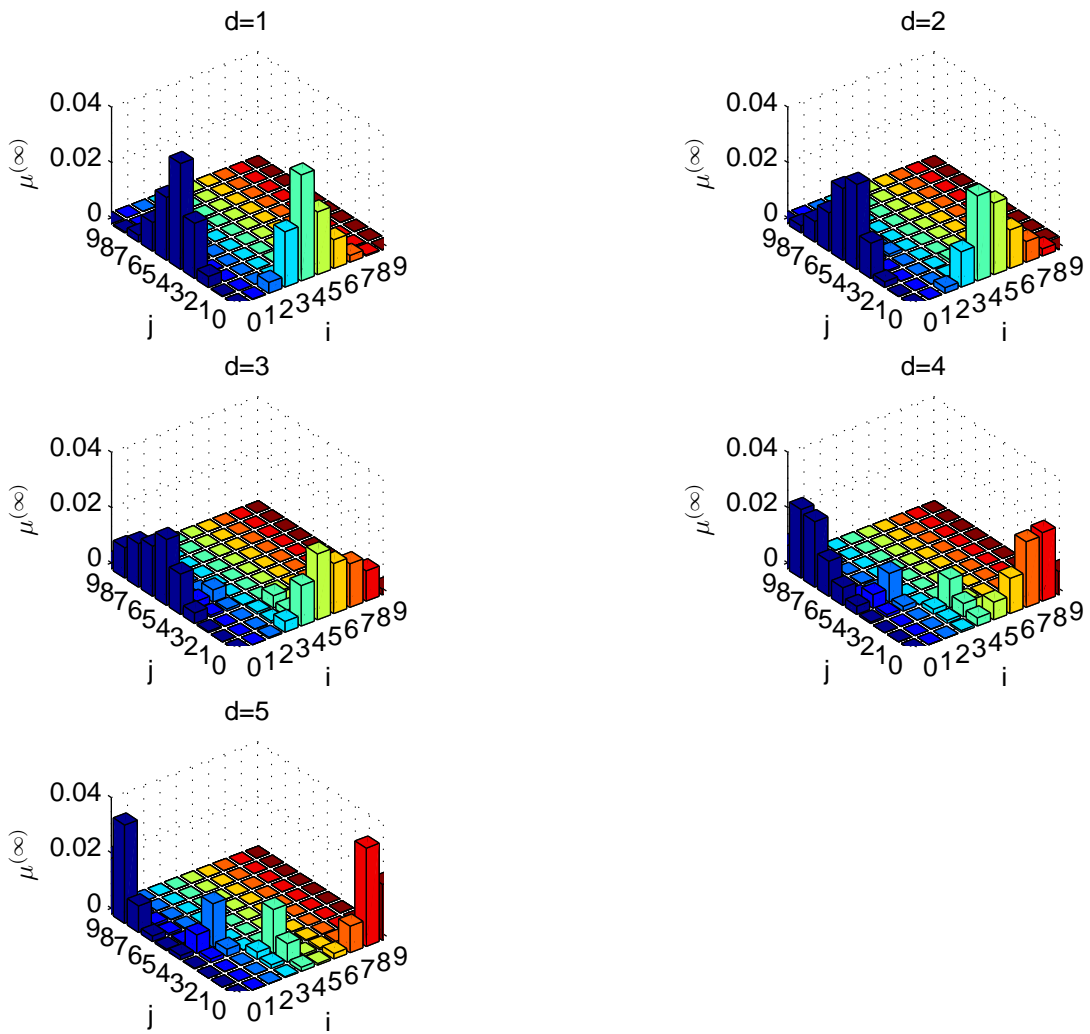
Figure 3: Limiting distribution \mu^{(\infty)} . Second equilibrium.
