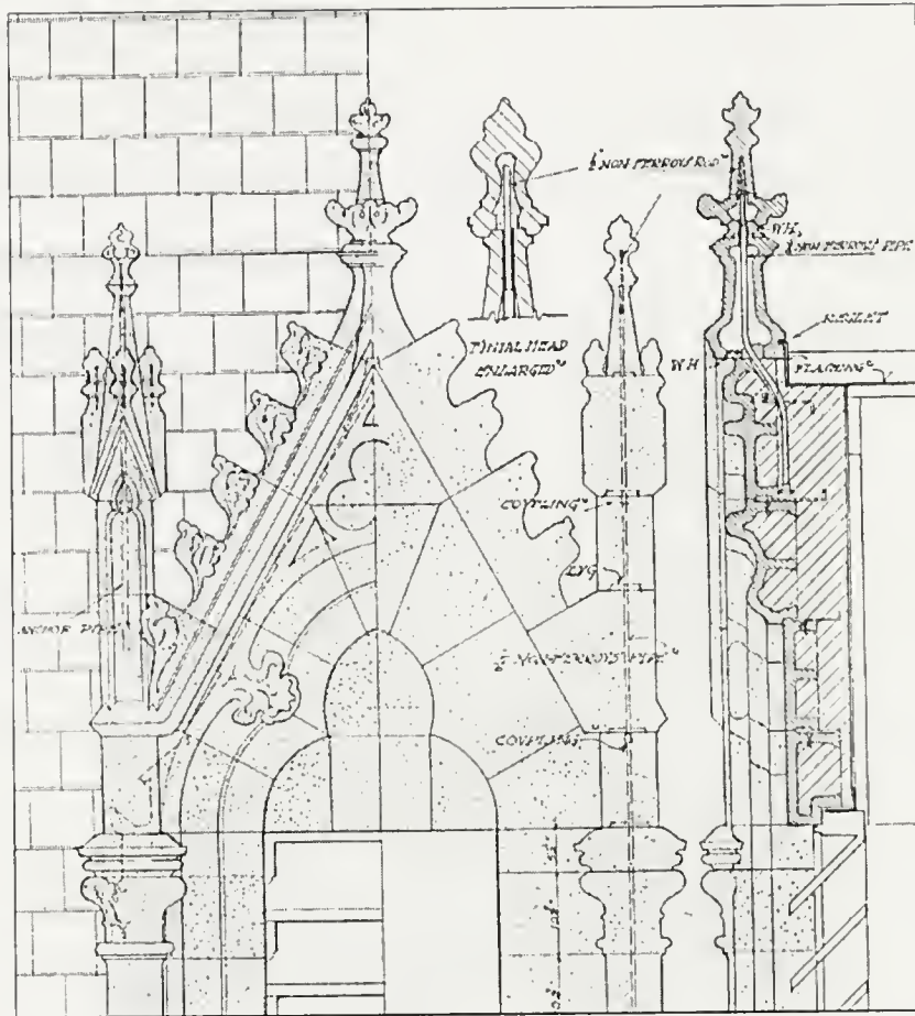
Standard Drawing 7: Taken from 'Louvered Dormer' plate no. 47 in Terra Cotta: Standard Construction (1927).
