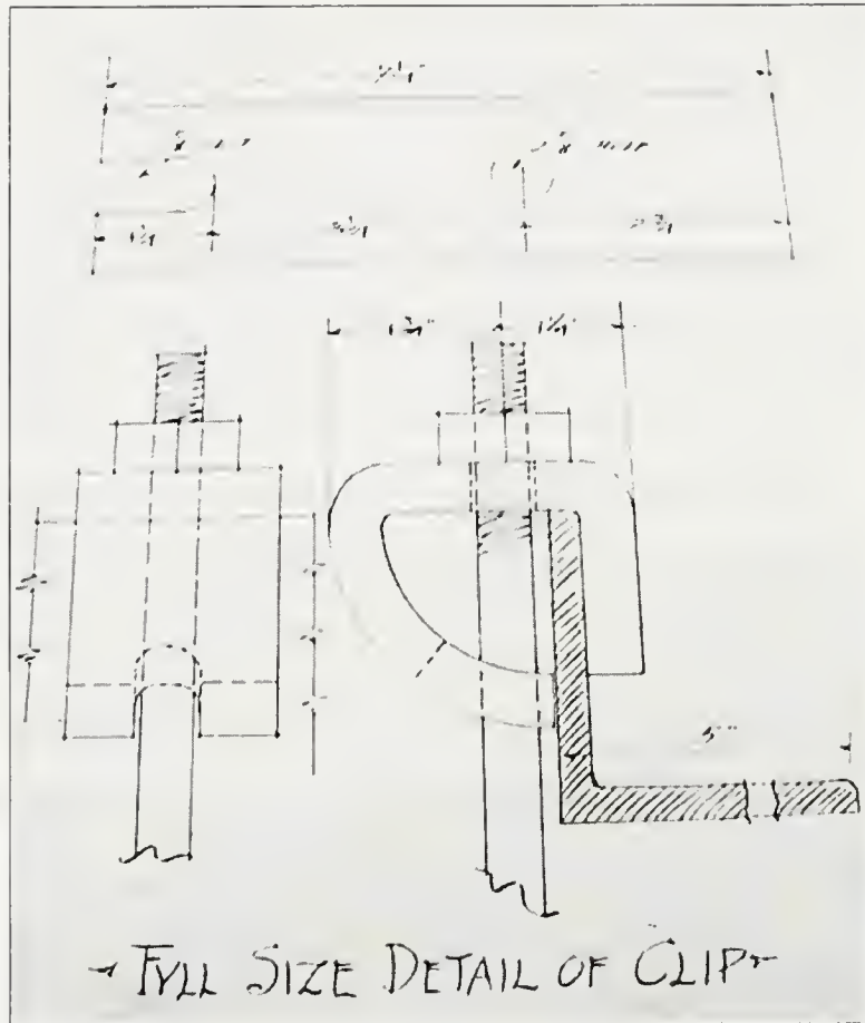
Example 7: City Hall, Chicago (1909). Northwestern Terra Cotta Company. Order 9001, Drawing 58308, Draffsman: Poulson
