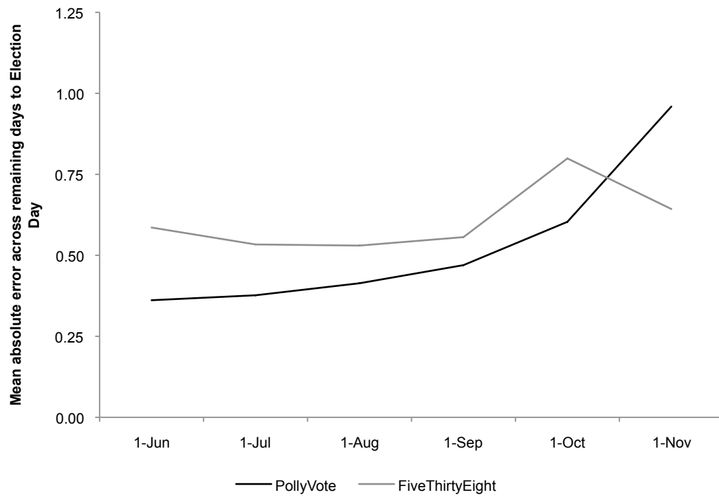
Figure 3: MAE of the PollyVote and FiveThirtyEight across the remaining days to Election Day 2012
