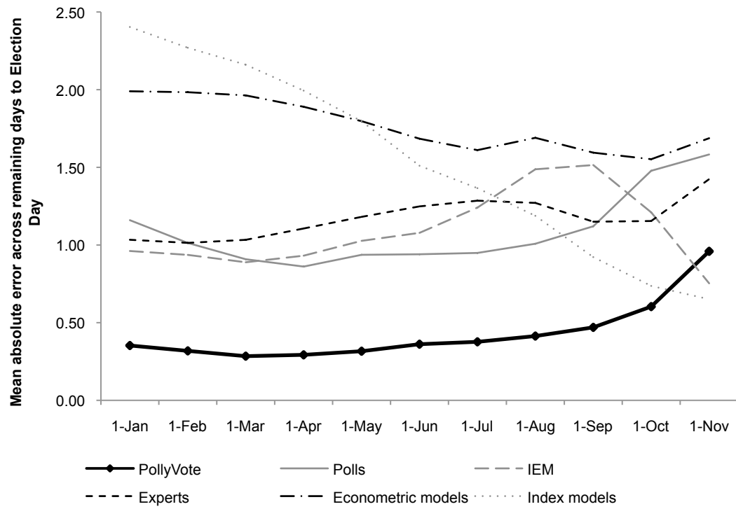
Figure 2: MAE of PollyVote and its components across the remaining days to Election Day 2012
