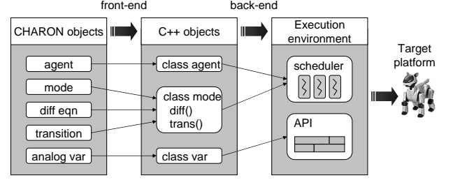
Figure 4: Code generator.
