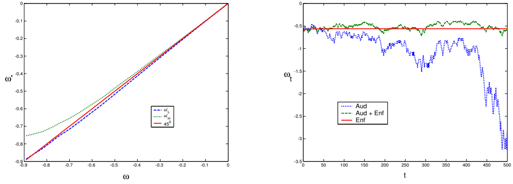
Figure 1.7: Left Panel: Continuation Promises, Right Panel: Sample Path \omega
