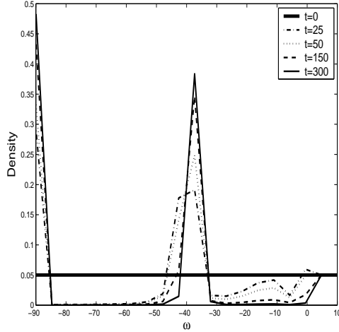
Figure 2.8: Density of \omega Over Time
