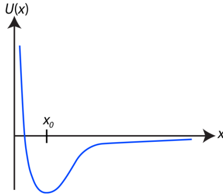
Figure 1-1 Schematic of the interatomic potential energy curve. The curvature of the potential energy minimum determines the (low-strain) elastic stiffness.
