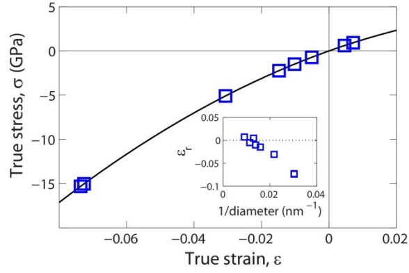
Figure 3-3 Estimation of relaxation strain \varepsilon_r along the NW axis. The provided inset shows increasingly compressive relaxation strains for NWs with smaller diameters. The bulk curve for Pd is plotted using the relation in Eq. 1 with D/E = -7.19 . The anomalous points indicating positive \varepsilon_r result from calculations with E values near the bulk value.
