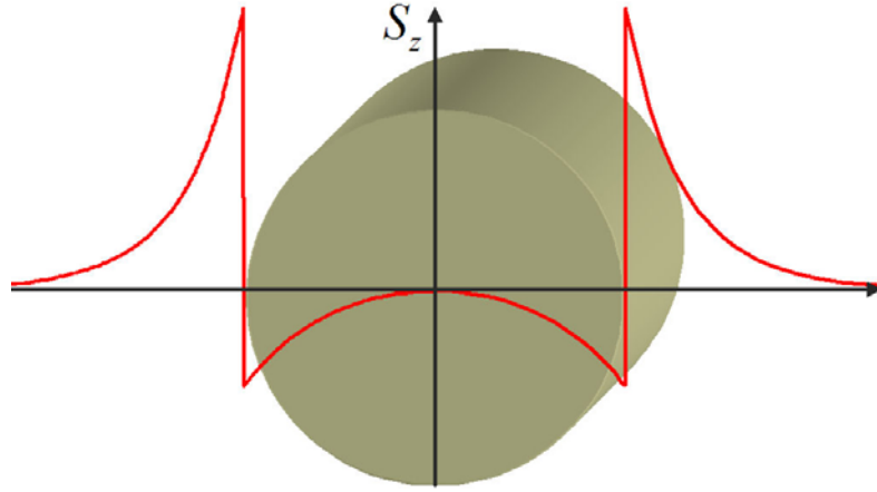
2 Figure 5 – Power flow distribution (real part of S_z , i.e., the Poynting vector component along the z axis) 3 for a nanowire supporting TM n=0 propagation. In this case, we have assumed \epsilon_1 = -3\epsilon_0 , a = \lambda_0/20 4 and therefore \beta = 6.91k_0 .
