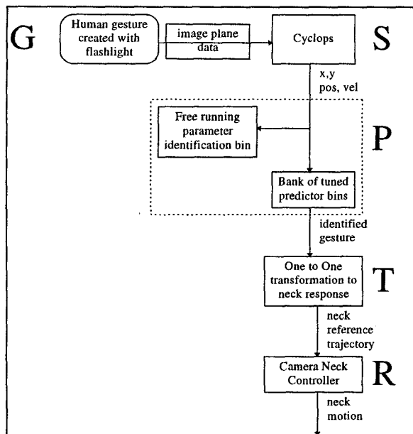
Figure 6: Gesture Recognition System Architecture
