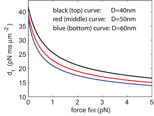
FIG. 4. (Color online) Drag coefficient per unit length as a function of the stretching force f_{\text{int}} at different channel widths D [calculated using Eqs. (11), (12), and (14)].
