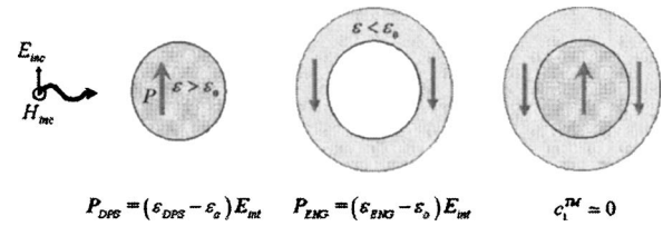
FIG. 4. Heuristic interpretation of the transparency phenomenon: cancellation of the overall dipole moment through an induced negative polarization vector.
