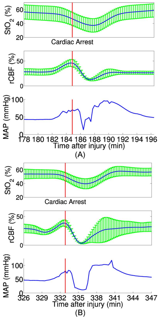
Fig. 6 Cerebral hemodynamic changes in a single animal during two episodes of apnea followed by cardiac arrest. (A) The onset of apnea produced the same StO_2 , rCBF, and MAP trends observed in Fig. 5. Cardiac arrest (solid vertical line) caused a significant decrease in MAP and rCBF, resulting in a further significant decrease in StO_2 . After ventilatory resuscitation, StO_2 , rCBF, and MAP gradually returned to preapnea levels. (B) The same “biphasic” dynamic change was observed during apnea in the same animal 2 h later. Error bars in StO_2 and rCBF represent standard deviation from large source-detector separations (1, 1.5, and 2 cm).
