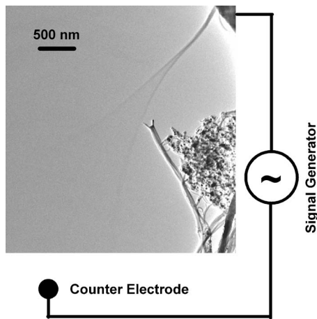
FIG. 1. Experimental setup. A SWNT bundle is actuated with an ac signal to induce vibration at its resonant frequency.
