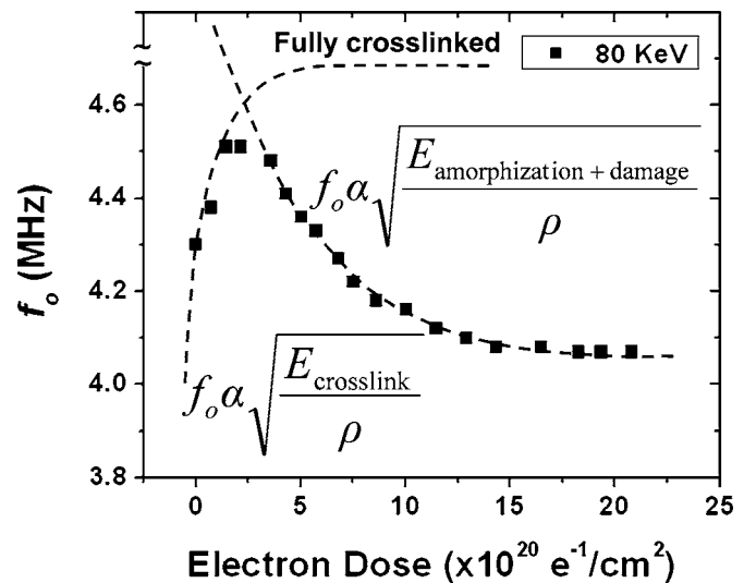
FIG. 2. Change in resonant frequency of a SWNT bundle as a function of electron irradiation dose taken from a SWNT bundle of D = 11 nm and L = 2.58 \mu\text{m} . The rate of change in f_o is a result of two competing mechanisms, cross-link formation and damage or amorphization in the structure. The effect of these mechanisms will be to increase and decrease the effective modulus, respectively (dashed curves). The plateau in the cross-linking case is based on the intuitive concept that, in the absence of damage, cross-linking will saturate and the SWNT bundle will behave as a monolithic beam.
