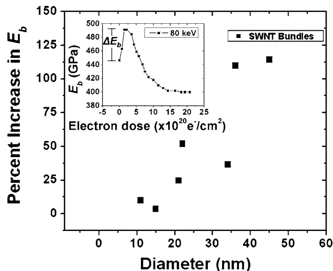
FIG. 3. Dependence of percent increase in E_b on SWNT bundle diameter. The bending modulus of a thin bundle was initially quite high, and E_b did not change much after the bundle was irradiated with an electron beam. For a larger diameter bundle, the initial E_b was low as a result of increasing shear flow in its structure. After irradiation, thicker bundles have shown higher percent increases in E_b , as the final E_b of the fully cross-linked bundles should be independent of diameter. The inset shows the evolution of E_b as a function of electron dose.
