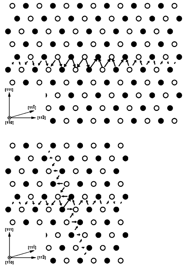
FIG. 10. Differential displacement maps of screw dislocation cores in iridium. In these figures, the circles depict atoms in the projection onto the plane perpendicular to the dislocation line ( 1\bar{1}0 ) and the open and closed circles distinguish two planes of atoms within one period. The arrows represent relative displacement parallel to the total Burgers vector between two neighboring atoms. The length of the arrows is proportional to the magnitude of the displacement normalized by a/2\sqrt{2} , where a is the fcc lattice parameter. (a) Planar core spread onto the (111) plane. (b) Nonplanar core spread onto the intersecting (111) and (11\bar{1}) planes.
