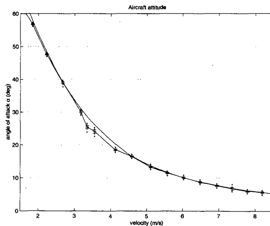
Figure 4: Experimental and model equilibrium manifolds. Angle of attack vs. velocity
