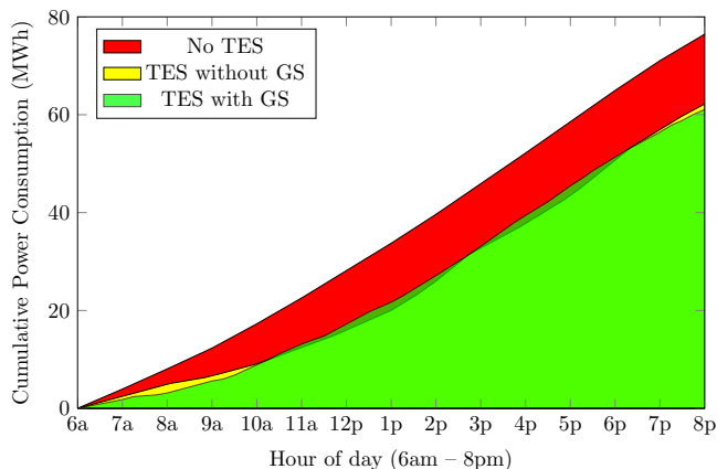
Fig. 10. Cumulative power plot showing that the total power consumption of Green Scheduling is the lowest followed closely by the TES without GS. The total consumption for no TES is quite high due to poor COP.
