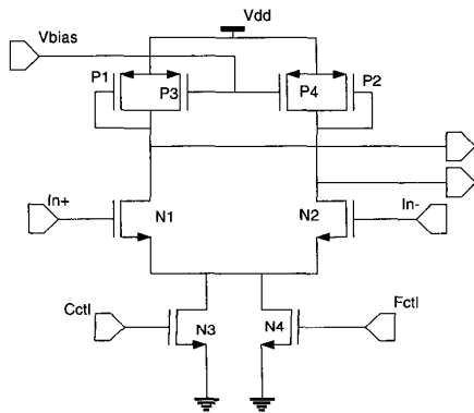
Figure 6. Delay Cell Circuit
