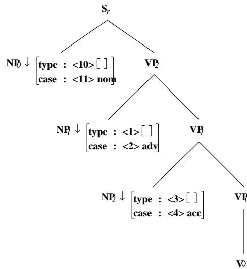
Figure 5.4: Declarative Tree: \alpha n x 0 n x p 1 n x 2 V
