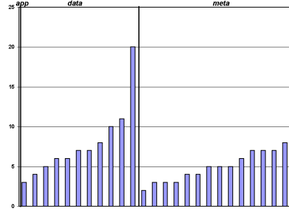
Figure 3: Longest simple path in non-recursive DTDs
