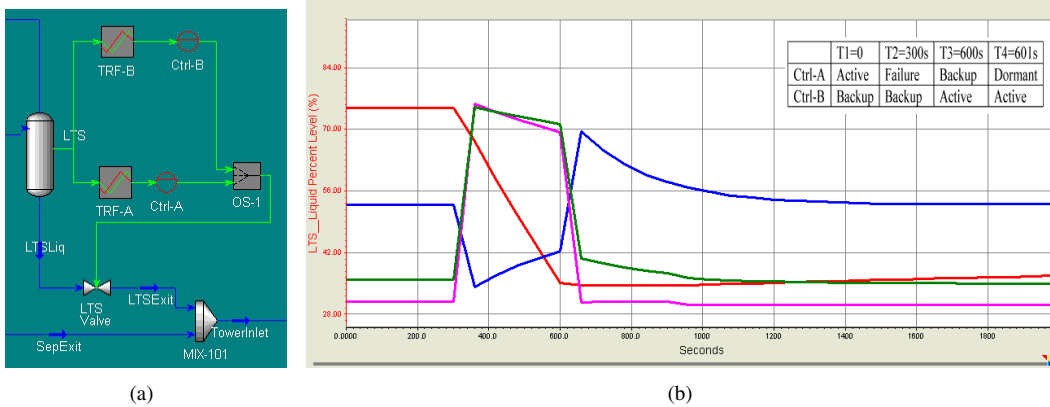
Figure 6. (a)Primary and backup controllers for the Low Temperature Separator. (b)Process control outputs during primary controller failure (300s), recovery (600s) and activation of backup controller (at 601s). Legend: LTS-Liquid Percent Level (red), SepLiq-Molar Flow (blue), LTSLiq-Molar Flow(magenta), TowerFeed-Molar Flow(green)
