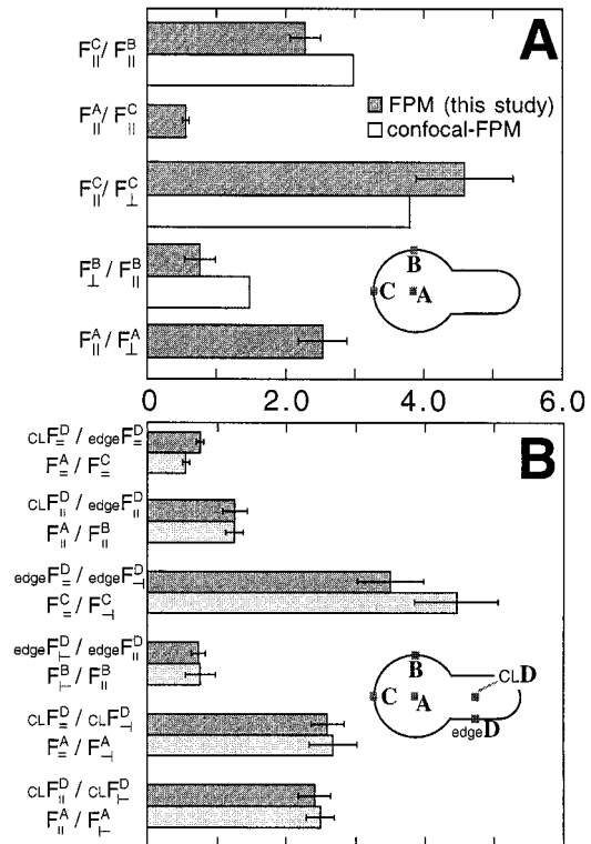
FIGURE 9 Polarization ratios for EMA-band 3-labeled ghosts aspirated into micropipettes. (A) Intensity ratios for points on the outer spherical segment of membrane. Ratios were averaged for like pairs of polarizers (six ghosts; averages \pm SD). Confocal FPM results of Blackman et al. (1996) (as estimated from Blackman's figure 5) are shown for comparison. (B) Intensity ratios at the midpoint of the aspirated projection, either at the centerline (CL) or at the edge, are plotted adjacent to homologous ratios from the outer spherical segment of membrane.
