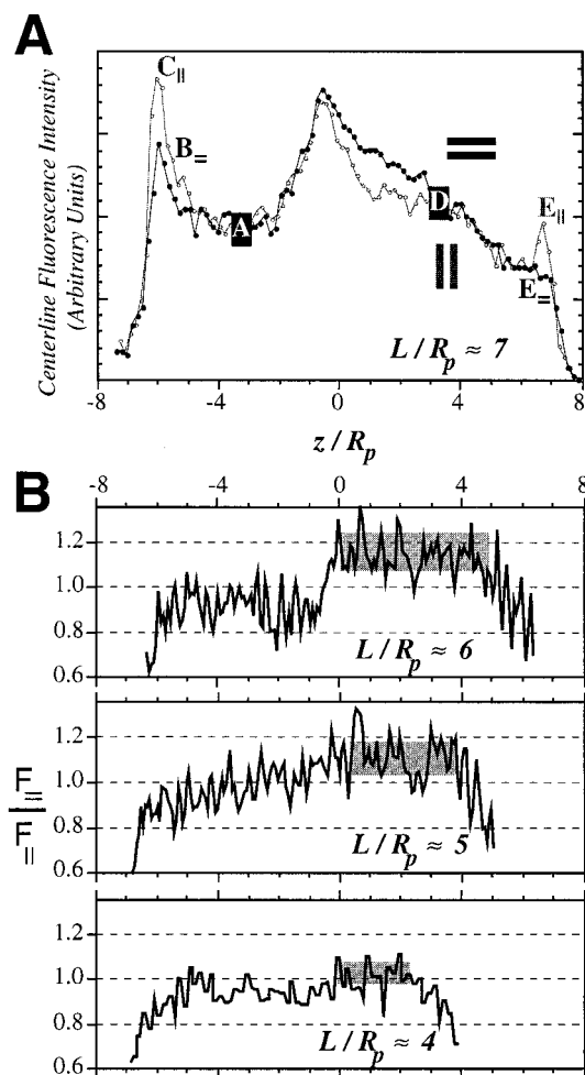
FIGURE 6 Centerline intensity profiles ( A ) or intensity ratios ( B ). Excitation and emission polarizers are parallel to each other, and both are either parallel ( \equiv ) or perpendicular ( \parallel ) to the micropipette axis. In A , R_p = 0.76 \mu\text{m} . The labeled points A and E represent, respectively, the center of the outer sphere or the tip of the aspirated projection. In B , a weak trend emerges for protofilament alignment in the network-stretched z direction. These regions are highlighted in gray; the projection's midpoint D is generally seen to be a good characteristic.
