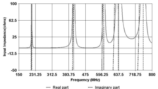
Fig. 5. Real and imaginary parts of the input impedance for the fifth iteration-order Hilbert antenna with feed point shown in Fig. 2.
