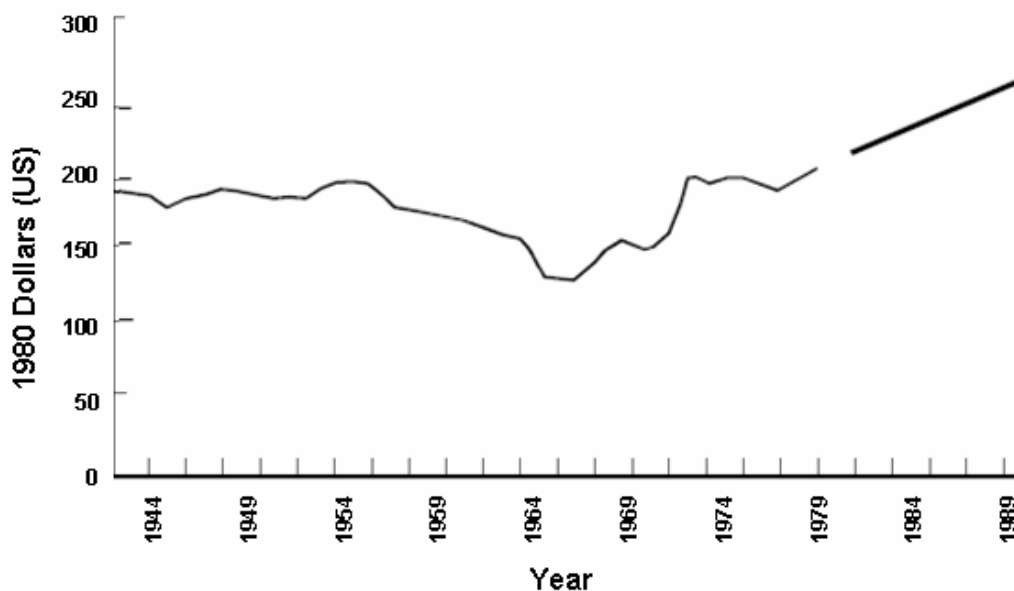
Figure 3. Chromium Prices: Holt's Forecast
