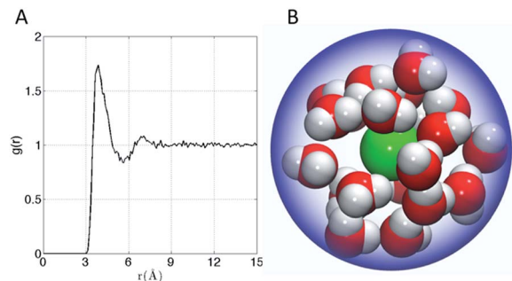
Fig. 6 (A) Water radial distribution function g(r) about Xe in water, where r is Xe–O distance. (B) Sampled configuration depicting first solvation shell (waters within 6 \text{\AA} ) of Xe in water.
