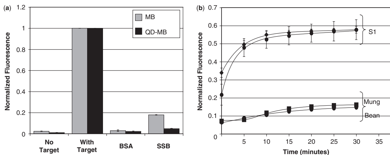
Figure 6. Fluorometric analysis of MB- and QD-MB-protein interactions and endonuclease degradation. (a) MBs and QD-MBs were incubated with molar excess of complementary target, BSA and SSB ( n = 3 each) and the peak fluorescent intensity of the MB was measured. SSB generated a false-positive signal upon binding to MBs and QD-MBs, although the increase in signal was much less pronounced with QD-MBs. (b) Incubation of MBs and QD-MBs with S1 endonucleases resulted in a significant increase in fluorescence. Both probes were degraded at similar rates. Mung Bean nuclease was also capable of degrading MBs and QD-MBs but to a much lesser extent than S1 nucleases. All fluorescent measurements were normalized to the signal elicited by MBs and QD-MBs, respectively, in the presence of saturating concentrations of complementary target.
