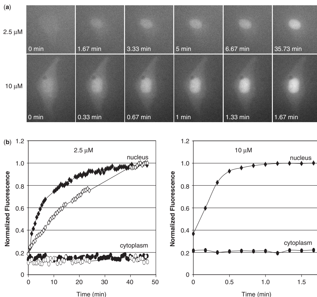
Figure 1. Nuclear localization of MBs. (a) Fluorescent microscopy images of MCF-7 cells microinjected with either 2.5\mu\text{M} or 10\mu\text{M} samples of MBs. The MBs are not perfectly complimentary to any known endogenous RNA in MCF-7 cells. An increase in fluorescence was observed in the nucleus shortly after injection in all cells analyzed. (b) The mean fluorescent intensity measured in the nucleus (filled diamonds) and cytoplasm (filled circles) was plotted as a function time. The fluorescent signal increased in the nucleus but not the cytoplasm. The rate of increase depended on the injected concentration of MBs. Higher concentrations of MBs led to a more rapid nuclear localization. When MBs were co-injected with 2'-O-methyl RNAs with the same targeting-sequence into MCF-7 cells, there was still an increase in nuclear fluorescence (open diamonds); however, the rate of increase in fluorescence was slightly slower. The fluorescent signal within the cytoplasm remained low (open circles).
