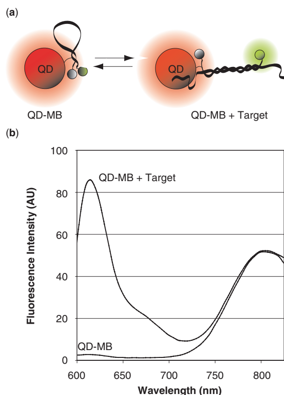
Figure 2. Schematic and emission spectrum of QD-MB conjugates. (a) Schematic of MB-QD conjugates in the presence and absence of target RNA. (b) The emission spectrum for 10nM QMBs (Cal610 reporter, Iowa Black RQ quencher, and a QD800 quantum dot) was recorded in the absence and presence of excess complementary oligonucleotide targets. The addition of complementary target led to a large increase in MB fluorescence; however, the QD fluorescence remained unchanged. This labeling ratio (prior to purification) was 6 MBs per QD for the QD-MB emission spectrum shown.
